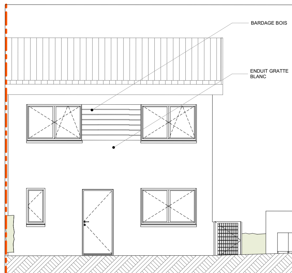
Façade principale
