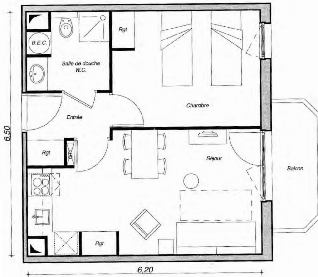
Plan T2 - Lot n°142 - R+1
