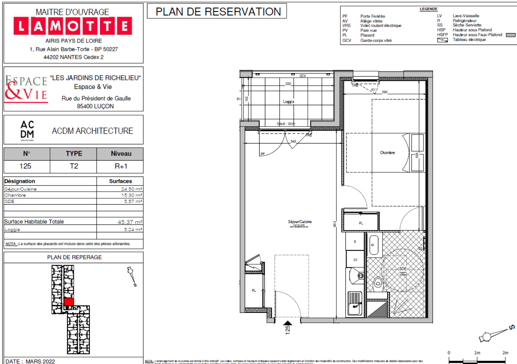
Plan T2 - Lot n°125 - R+1
