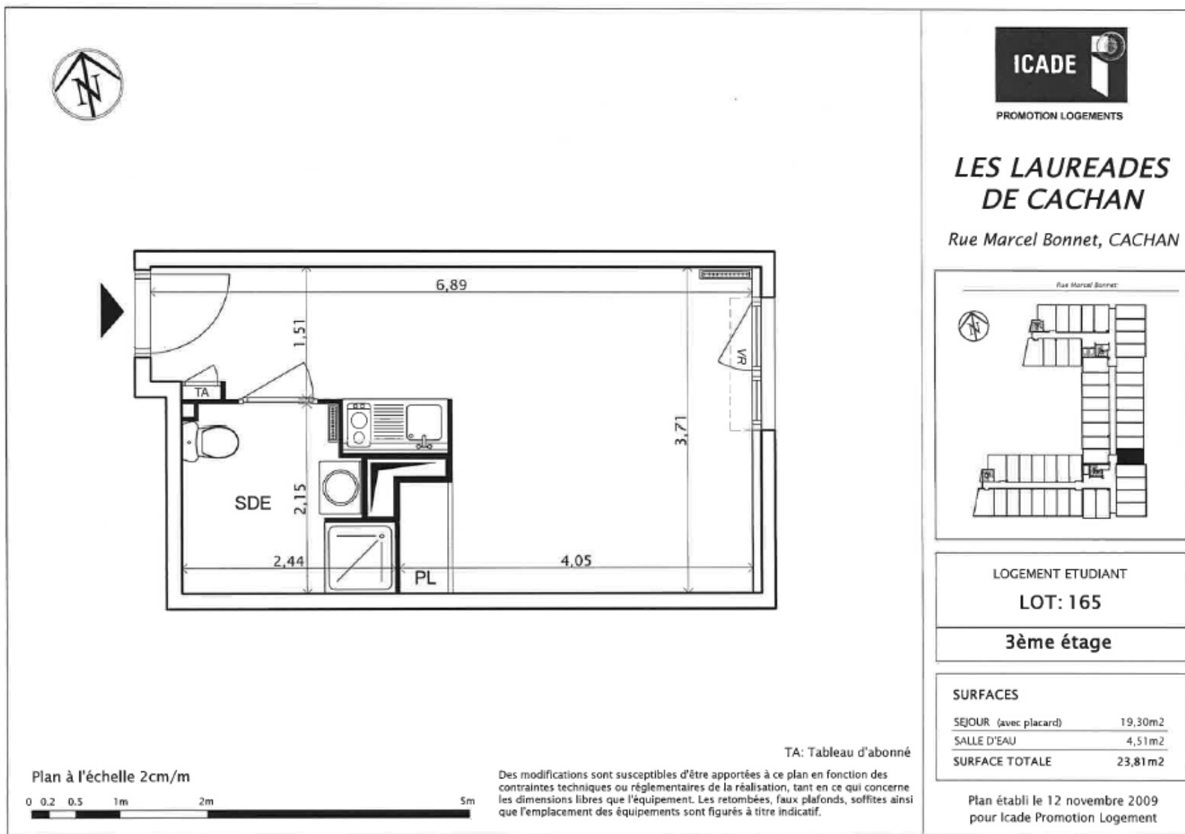
Plan Studio - Lot n°165 - R+3
