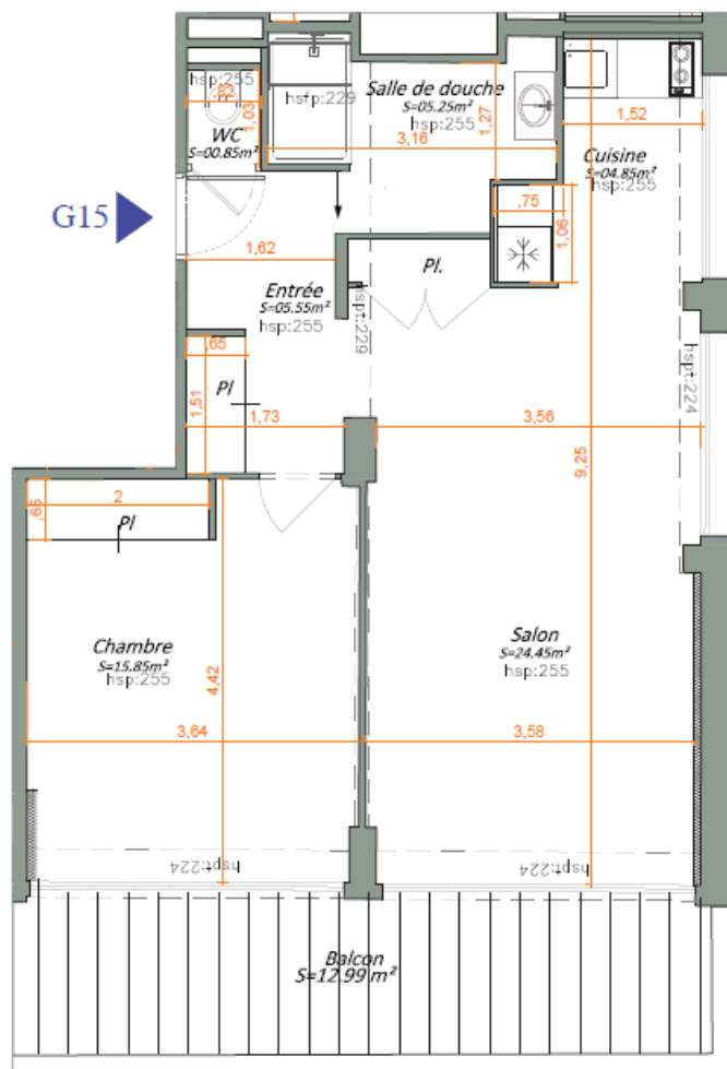
Plan T2 – Lot n°G15 – R + 1
