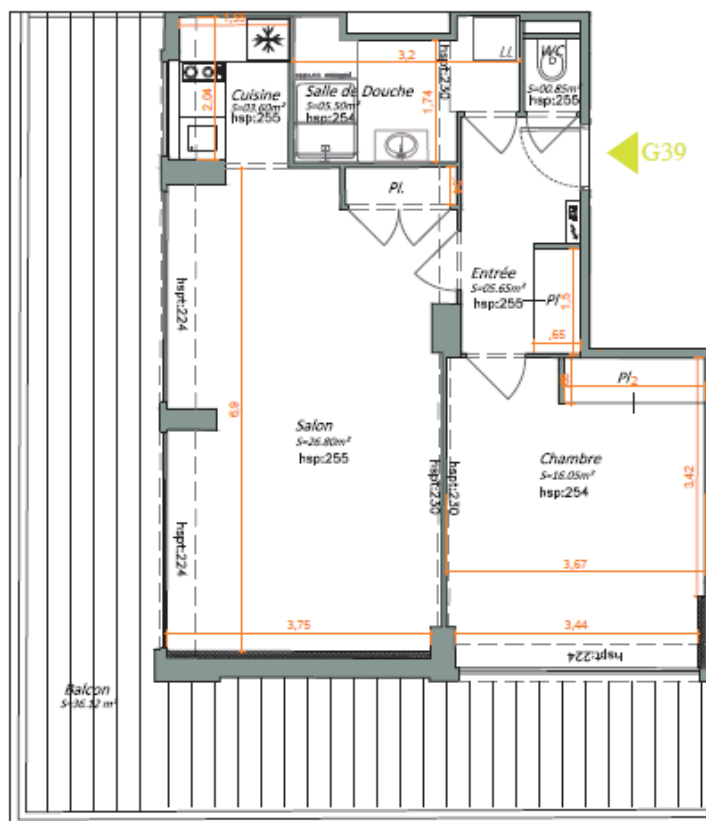
Plan T2 - Lot G39 - R+3
