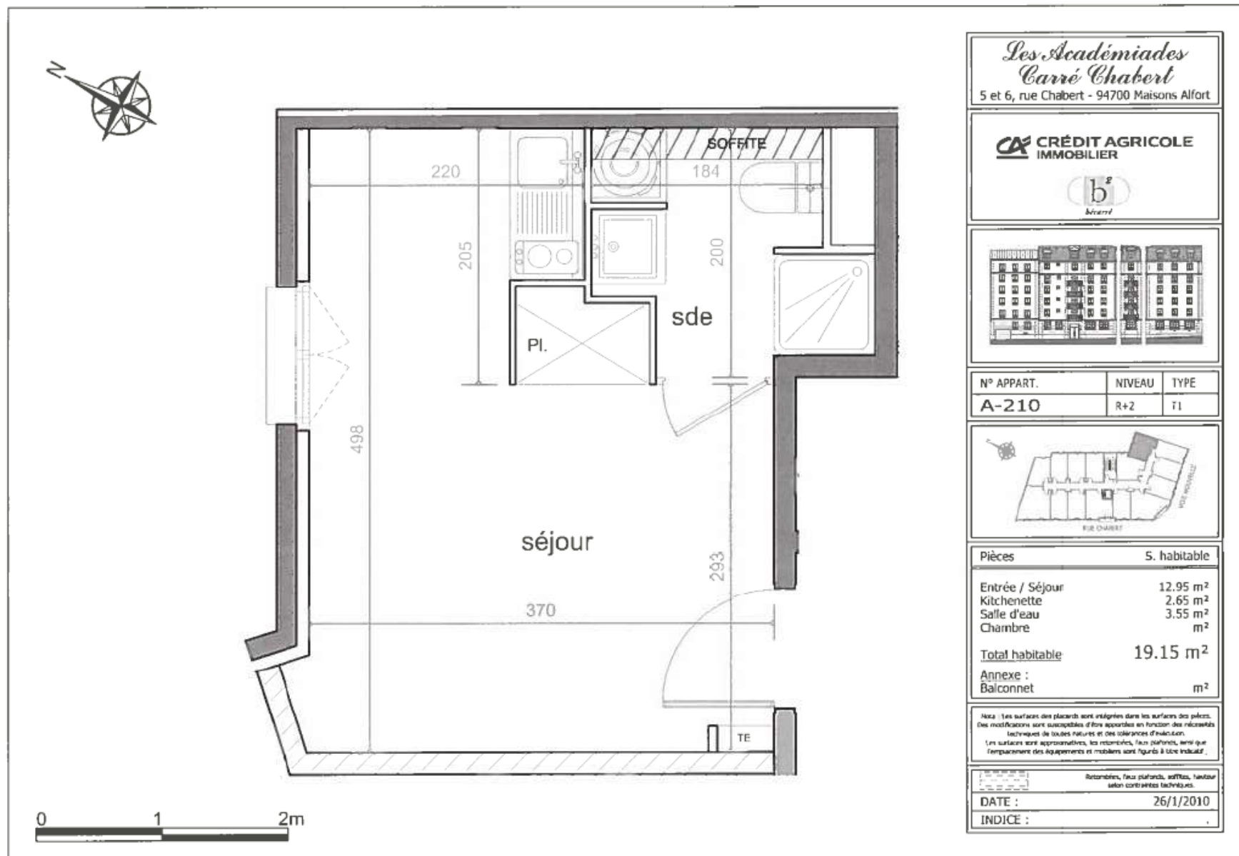
Plan Studio - Lot n° 210 - R+2
