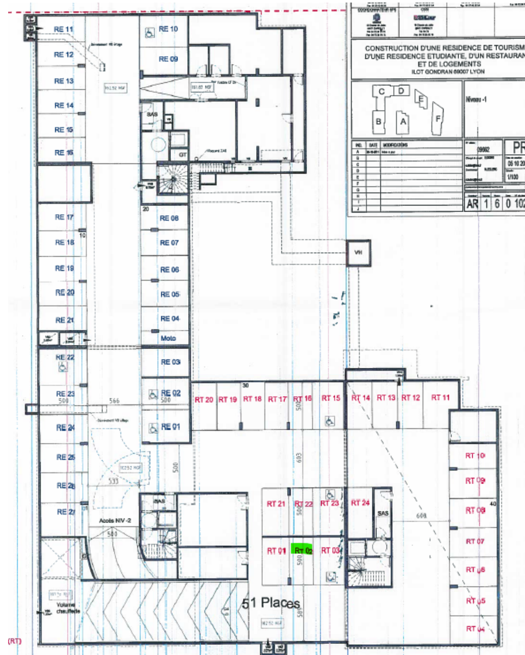
Plan Parking
