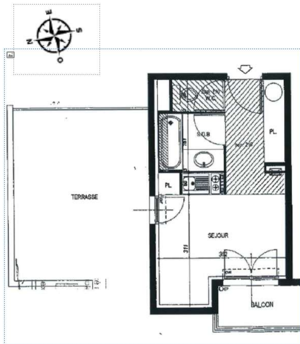
Plan Studio - Lot n°119 - R+2
