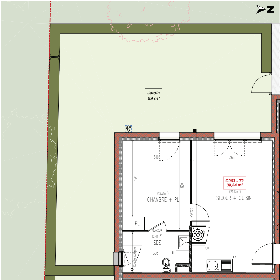
Rez-de-chaussée - C003
