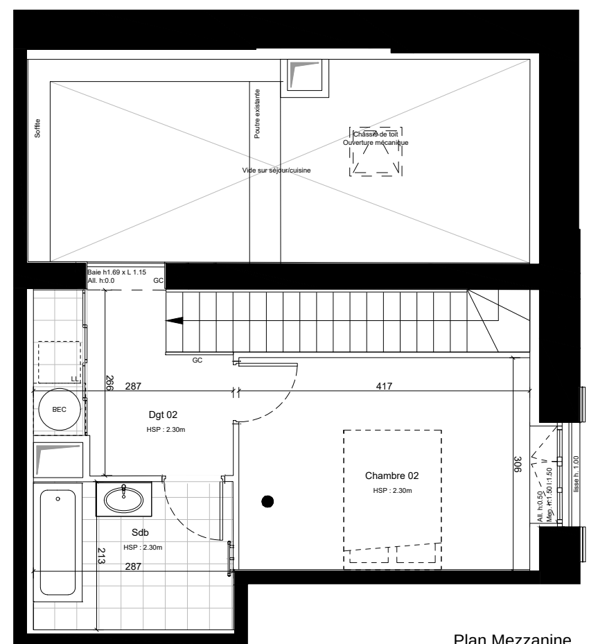
Plan Mezzanine
