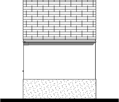
Façade ARRIERE
