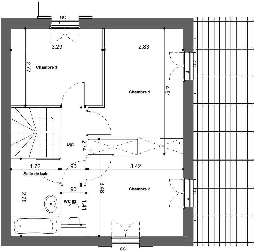
PLAN R+1
