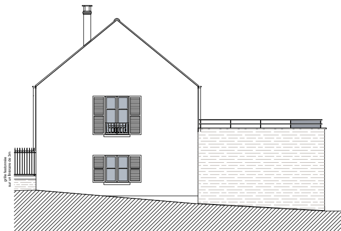
FACADE SUD
