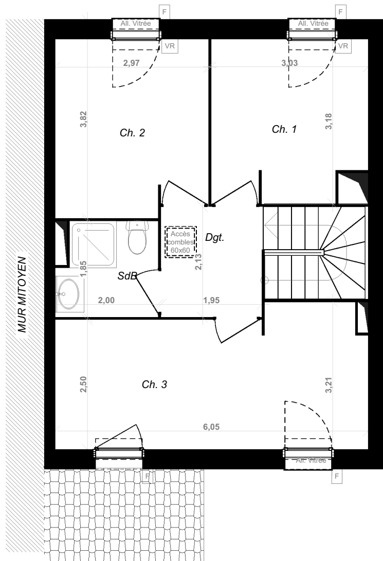
PLAN R+1
