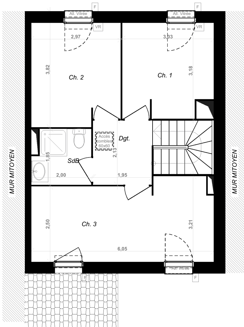
PLAN R+1
