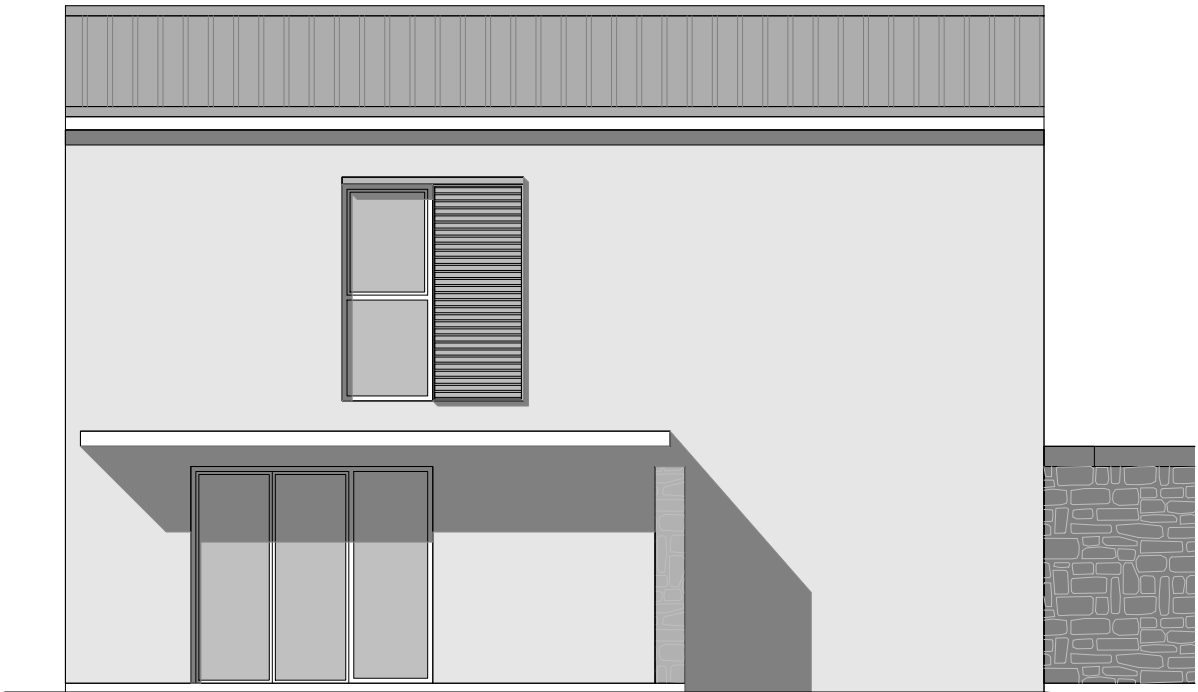
FACADE SUD
